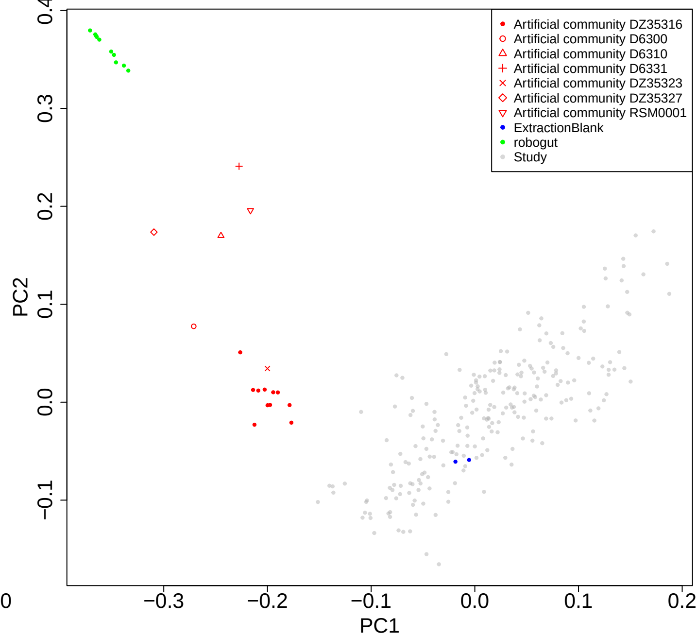
Weighted UniFrac
