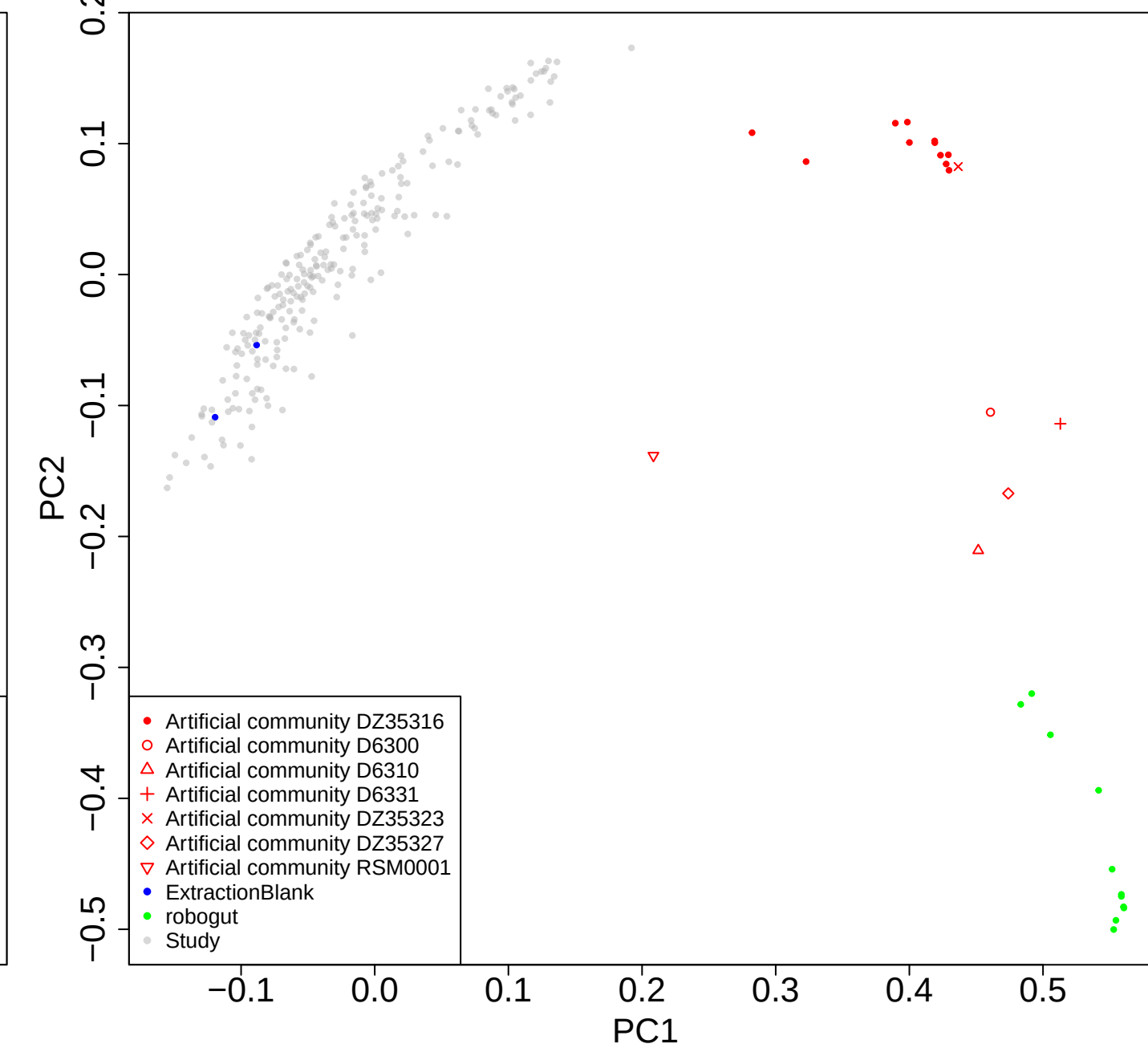
Unweighted UniFrac
