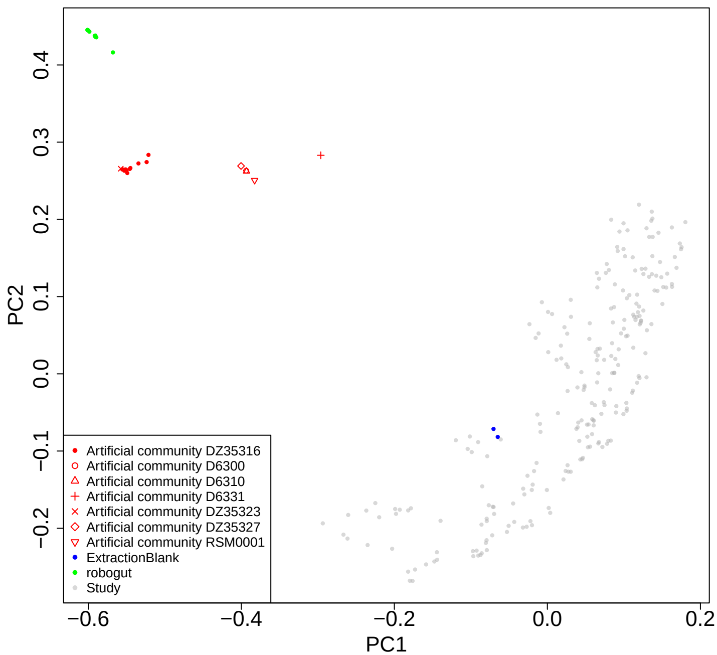
Bray Curtis
