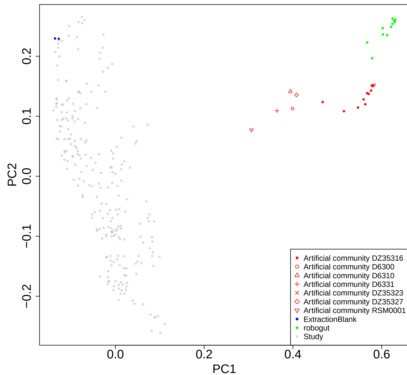
Jaccard
