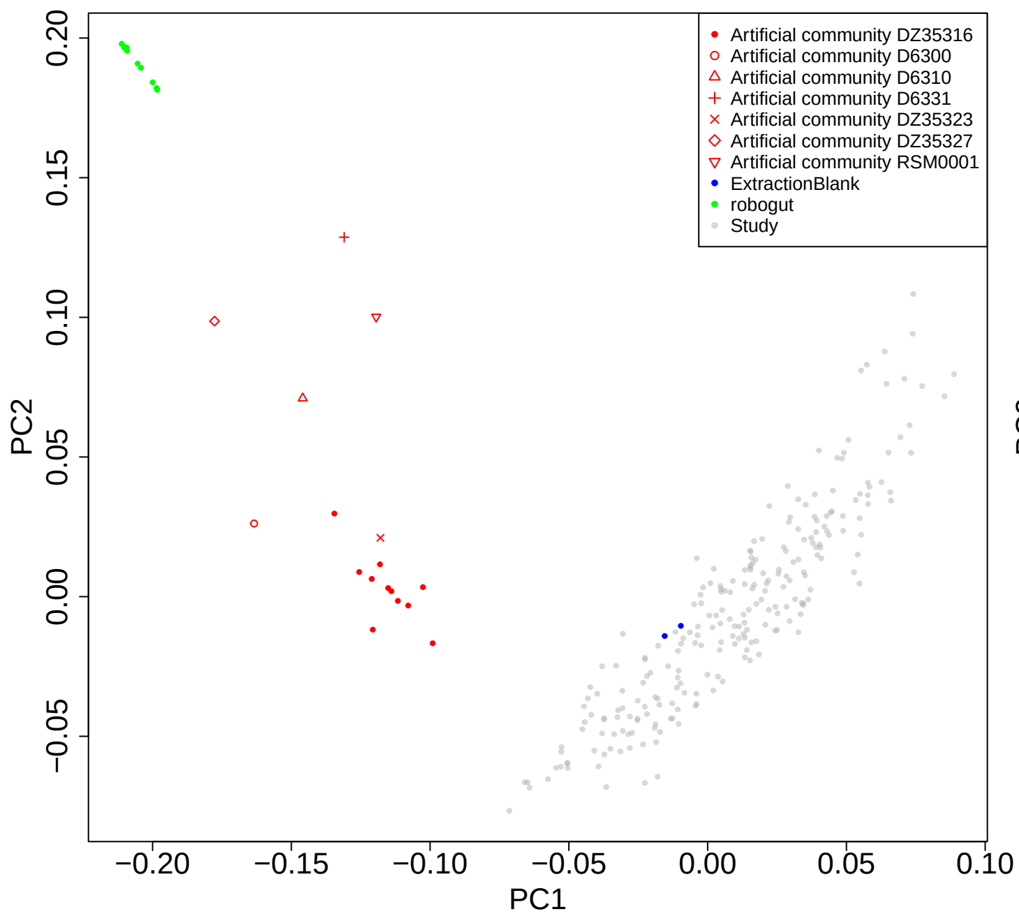
Generalized UniFrac
